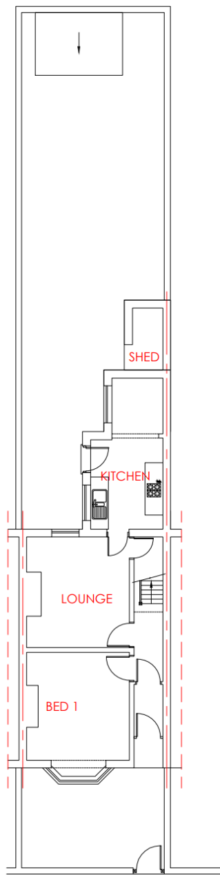
EXISTING PLAN G & SITE PLAN SCALE 1:50
