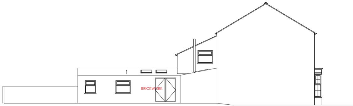
PROPOSED SIDE ELEVATION SCALE 1:50
