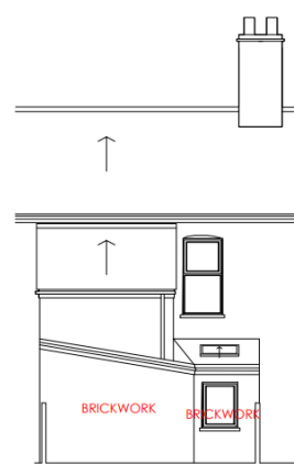
PROPOSED REAR ELEVATION SCALE 1:50
